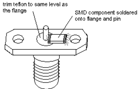
SMA Fixture: Mount SMD components onto SMA connector
