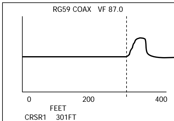
Open End – Pulse TDR
